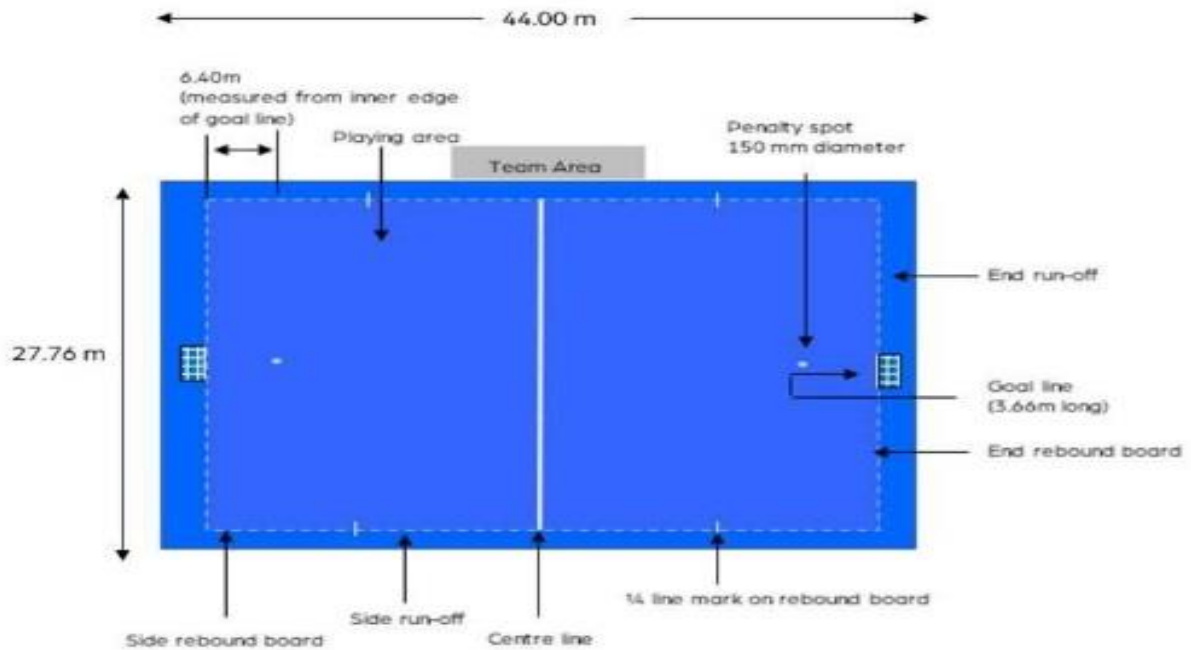
Figure 1 – Category 1 court layout
